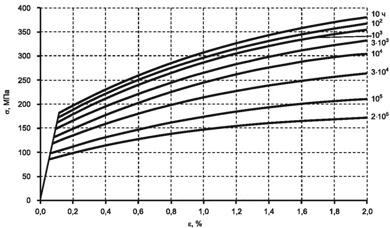
б) При T = 723 \text{ K} ( 450 \text{ }^{\circ}\text{C} )
