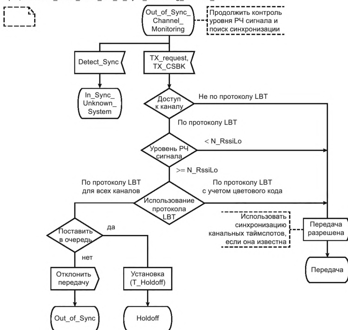
Процесс TDMA_Direct_Mode_Out_of_Sync_Monitoring_Channel_Access
